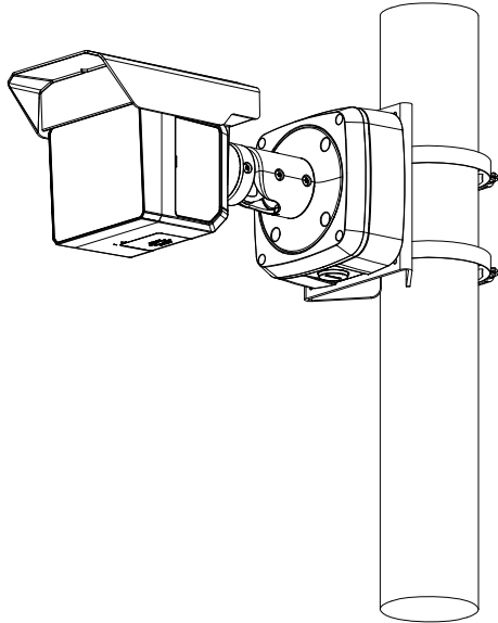
Pole Mount(Vertical)
