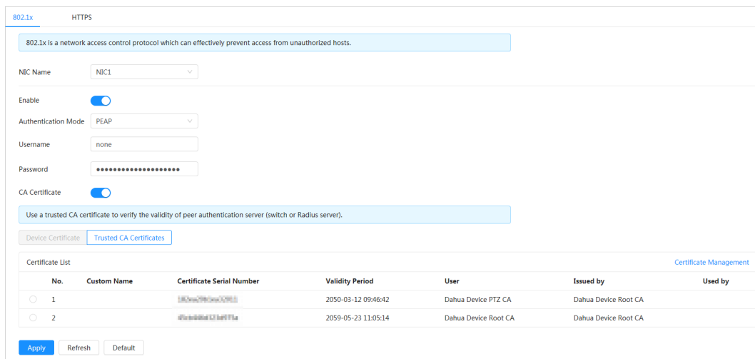
Figure 10-3 802.1x (PEAP)
