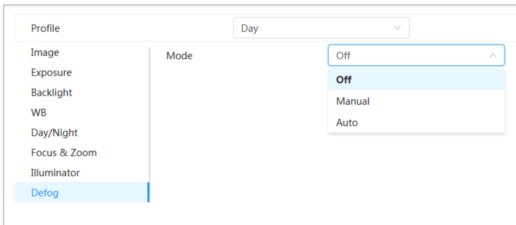
Figure 4-14 Defog
