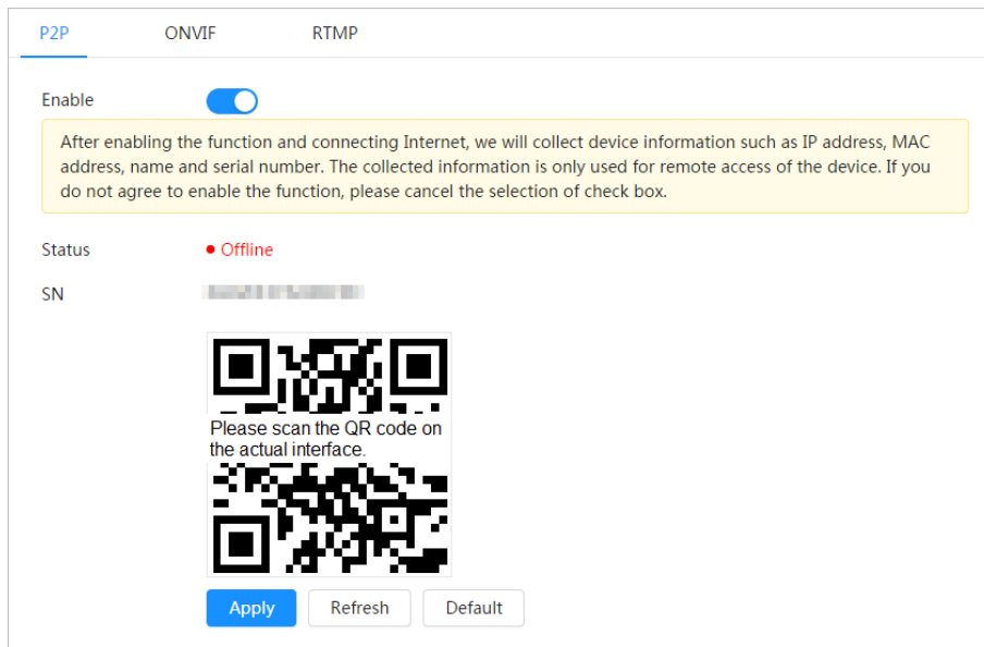
Figure 4-44 P2P
