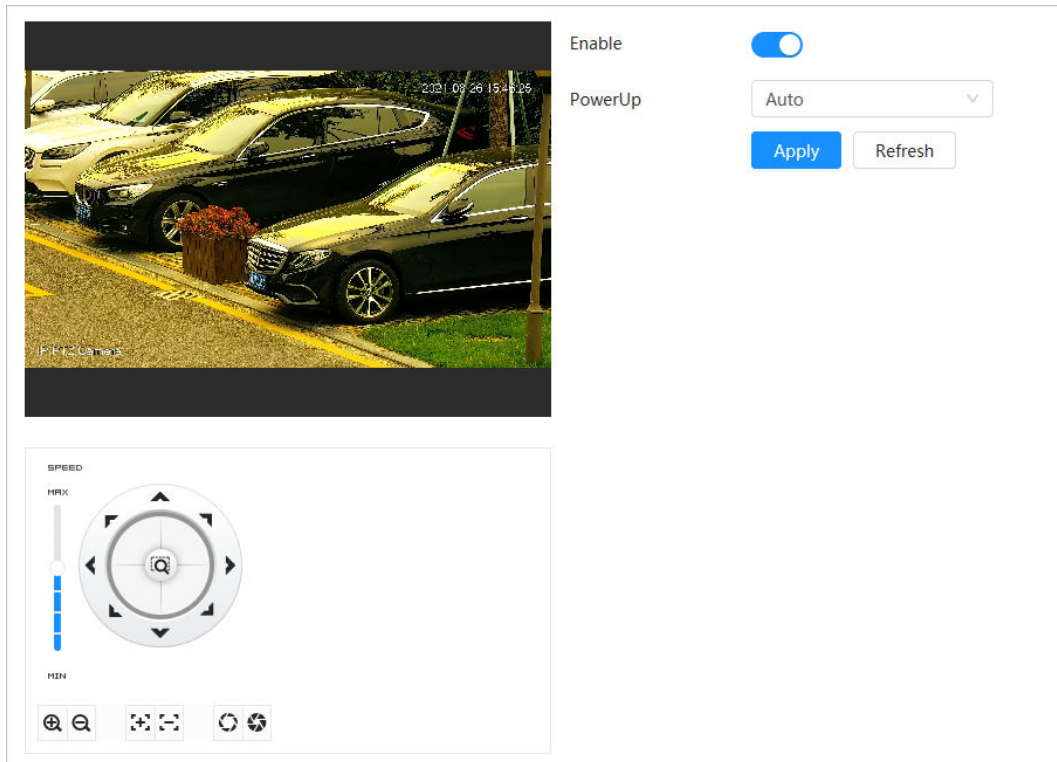
Figure 4-55 PowerUp
