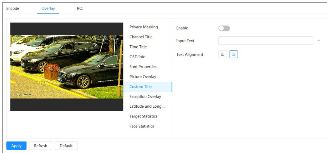
Figure 4-22 Custom title
