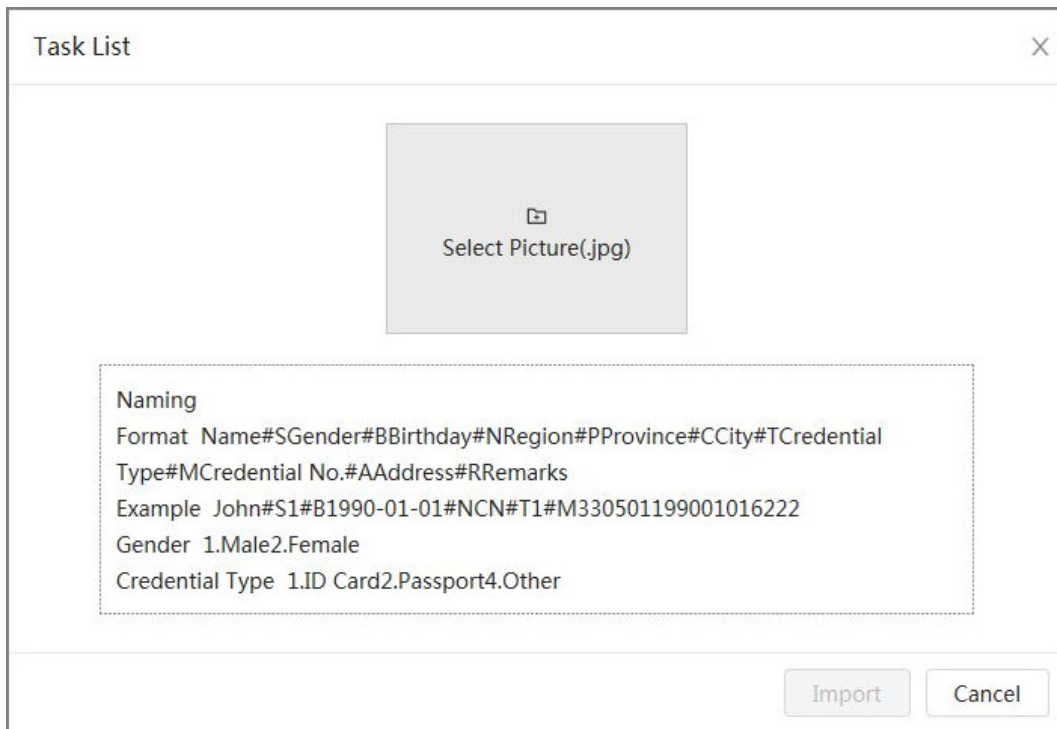
Figure 9-8 Task list
