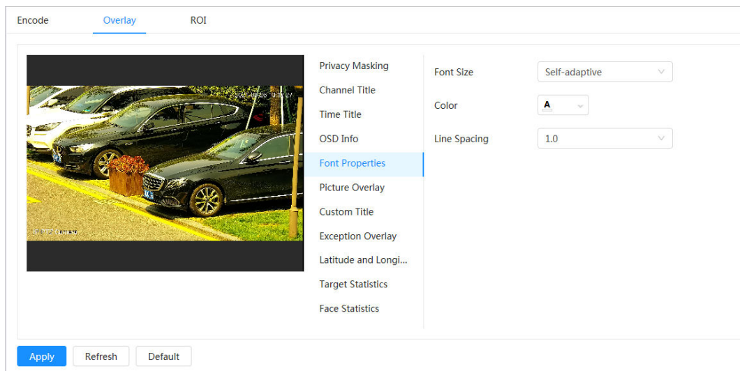
Figure 4-20 Font properties
