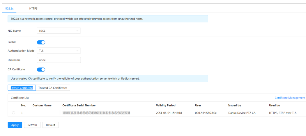
Figure 10-4 802.1x (TLS)
