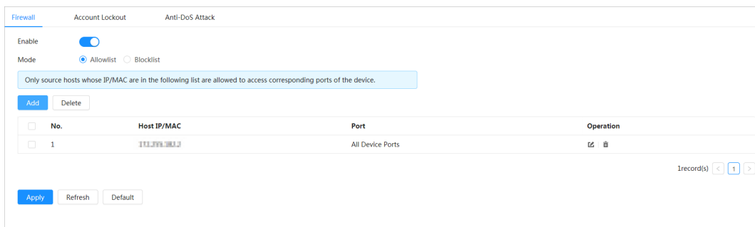
Figure 10-6 Firewall
