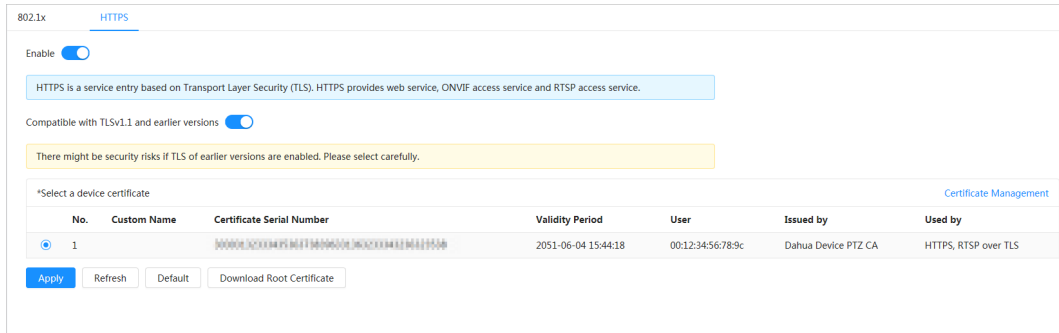
Figure 10-5 HTTPS
