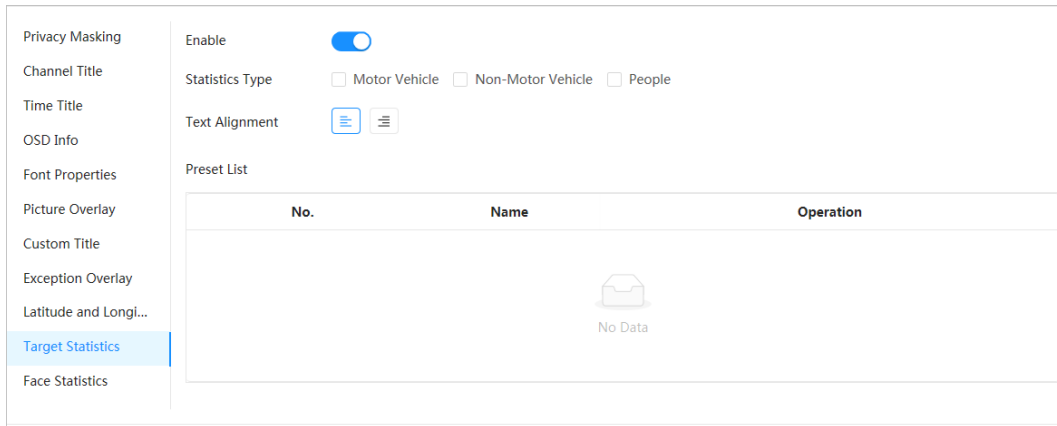
Figure 4-25 Target statistics
