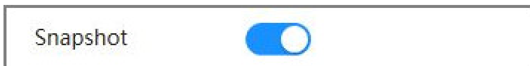
Figure 4-65 Snapshot linkage
