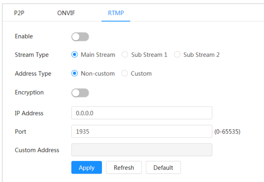
Figure 4-46 RTMP
